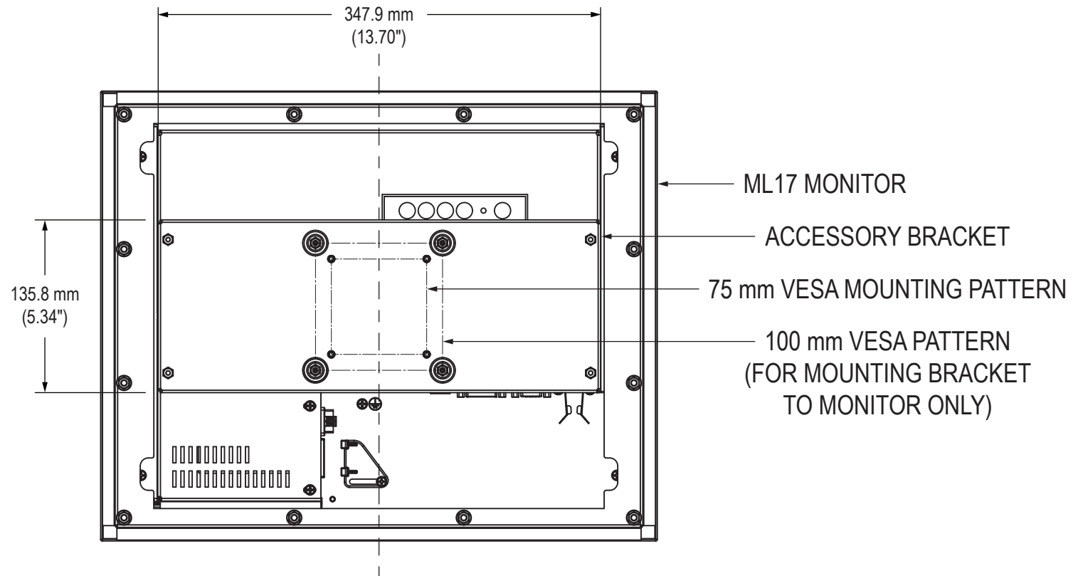
Rear View
